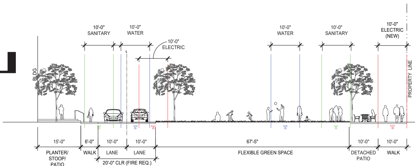
SECTION A
