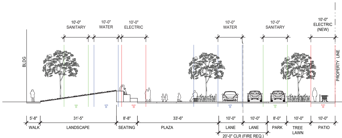
SECTION C
