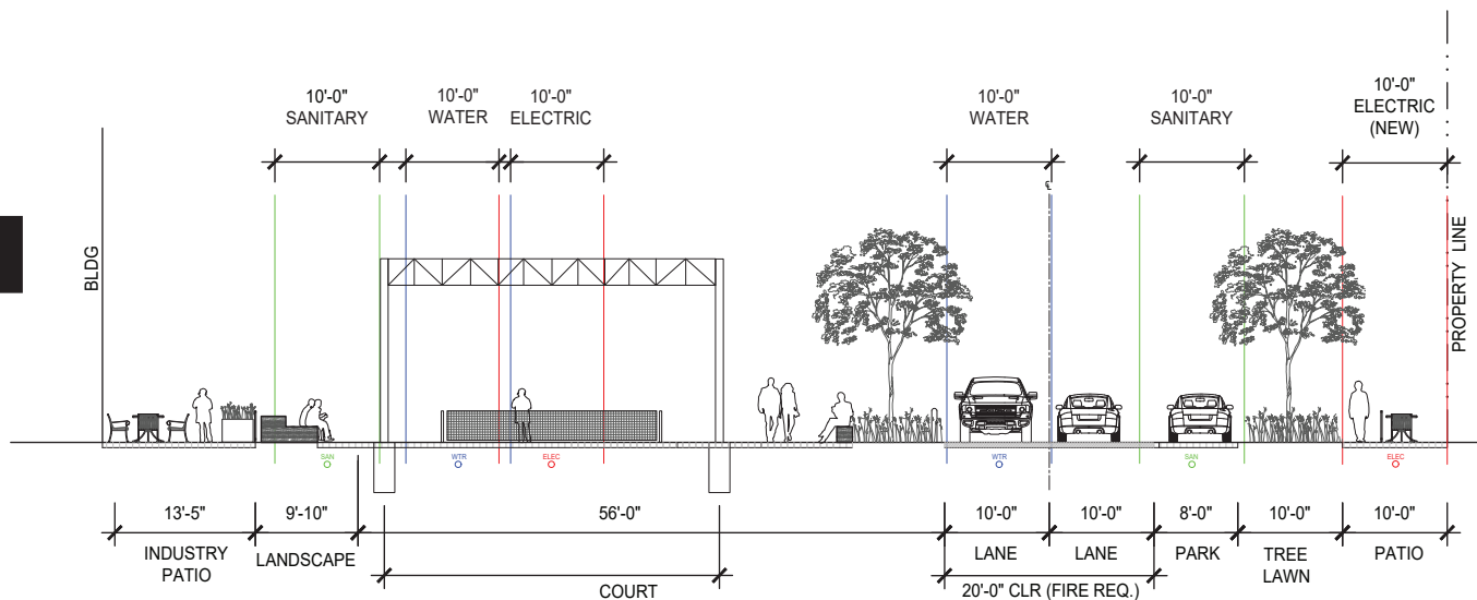
SECTION B
